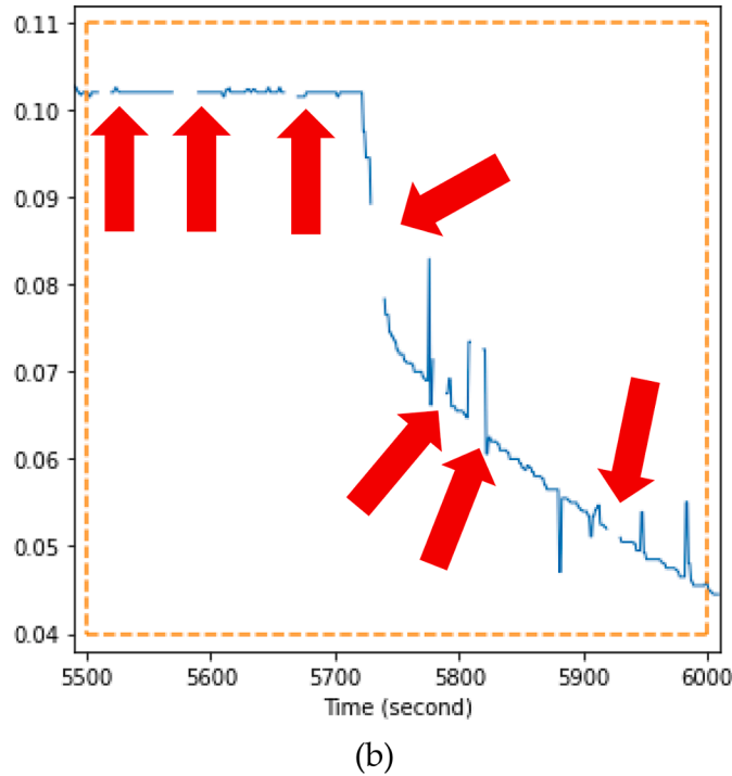
Fig. 15. Results prior to mitigation and interpolation. (a) Denoised signal before mitigation and interpolation. (b) The zoomed-in perspective of (a) in orange dashed rectangle. Red arrows point to the gaps of discarded windows.
