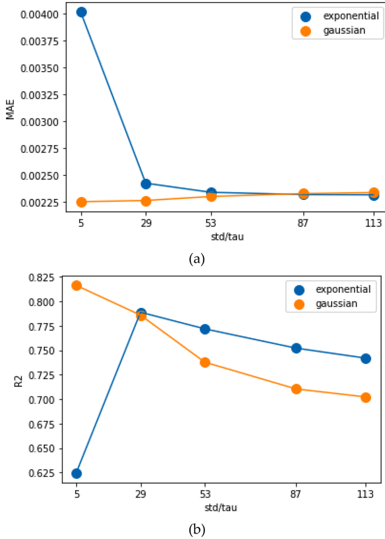
Fig. 22. . AE and R2 comparison for extended configuration. (a) MAE at extended std/tau settings. Lower is better. (b) R2 at extended std/tau settings. Higher is better.
